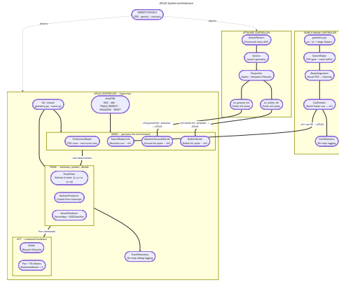
Figure 2: ATLAS system architecture diagram
